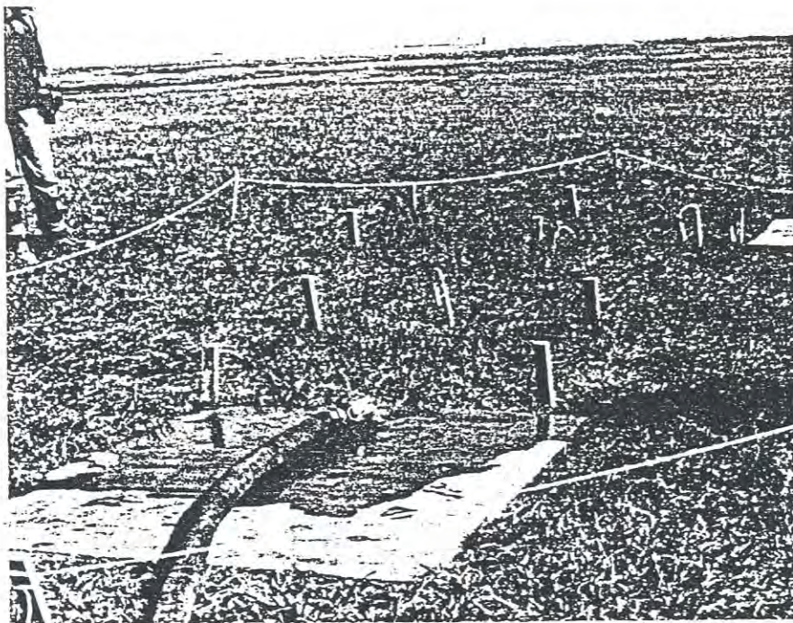
Figure 3. Application of seawater at the West Dock mesic site. The plastic tubes attached to the lysimeters can be seen at the center and the right.
