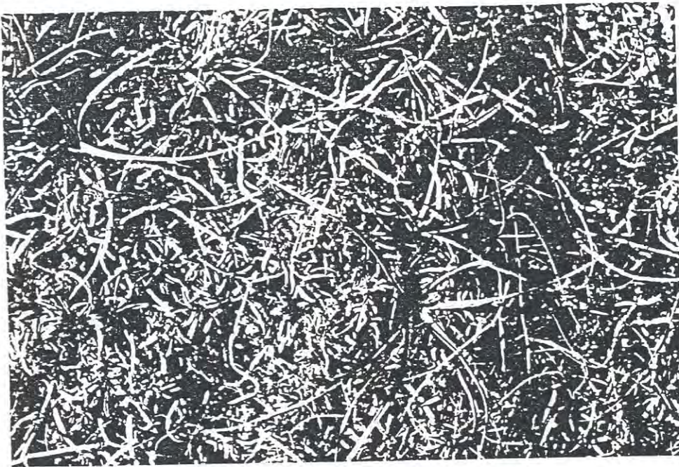
d. Experimental plot at the Drill Site No. 2 mesic site. The gray color is primarily due to dead Dryas integrifolia . The live vegetative cover decreased from 107% in 1980 to 26% in 1981 at this site.
