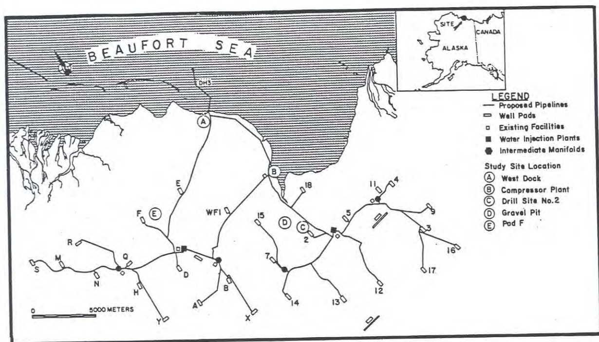
Figure 1. Locations of the seawater spill study sites.
