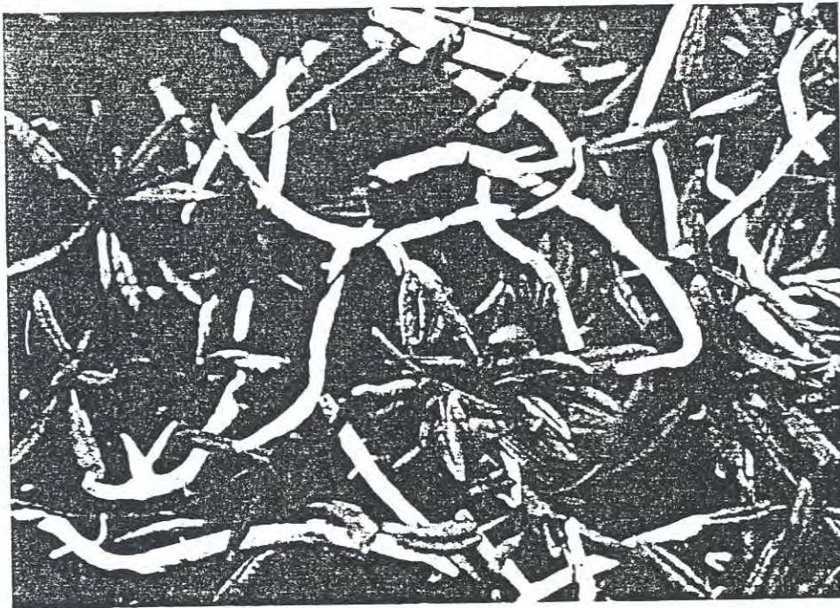
j. Leaves of Dryas integrifolia in an experimental plot at the Drill Site No. 2 mesic site in 1981. These plants produced no new foliage in 1981.
