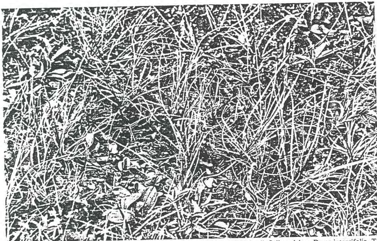
b. Vegetation at the Pad F mesic site. The dominant plants are Carex bigelowii , Salix pulchra , Dryas integrifolia , Tomentypnum nitens and Oncophorus wahlenbergii . (Photo by Sue Degler.)
