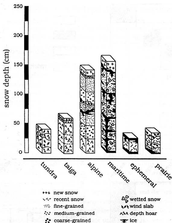
Figure 2.38. Basic stratigraphy and texture for each snow class in Sturm et al.'s climatic classification, as found in mid-to-late winter (after Sturm et al., 1995).
