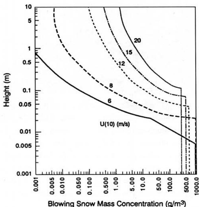
Figure 2.4. Vertical profiles of blowing snow mass concentration as a function of wind speed (after Pomeroy and Male, 1992).
