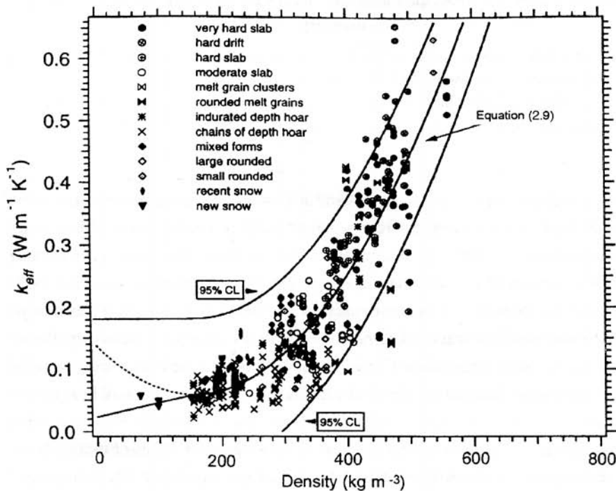
Figure 2.25. Effective thermal conductivity of snow as a function of snow crystal type and snow density, along with Equation 2.9 plotted with its confidence intervals (CL). For a discussion of snow crystal classification, see Section 2.4 in this chapter (after Sturm et al., 1997).
