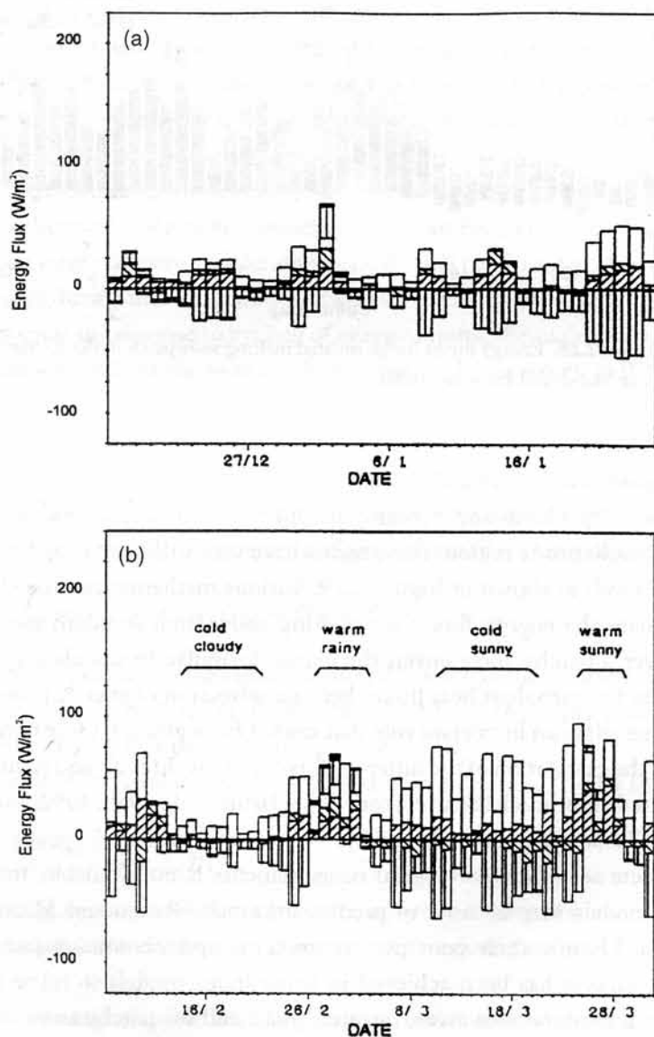
Figure 2.29. Daily variation of energy balance components of an alpine snow cover in the French Alps during three periods: (a) midwinter, (b) late winter, and (c) spring.
