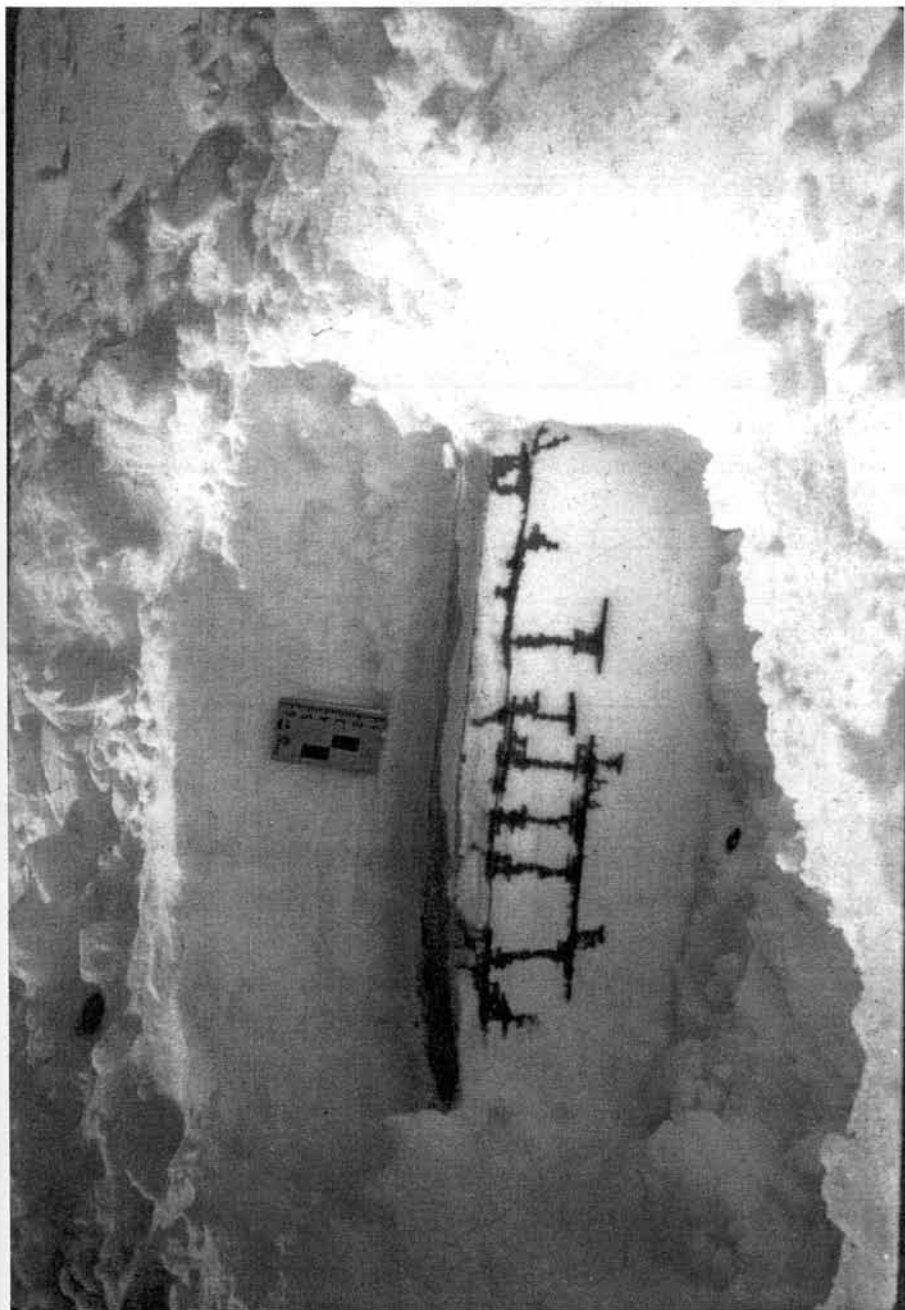
Figure 2.34. Photograph showing dye injection into developing flow fingers and wet layers in cold arctic snow (by Phil Marsh, NHRI).
