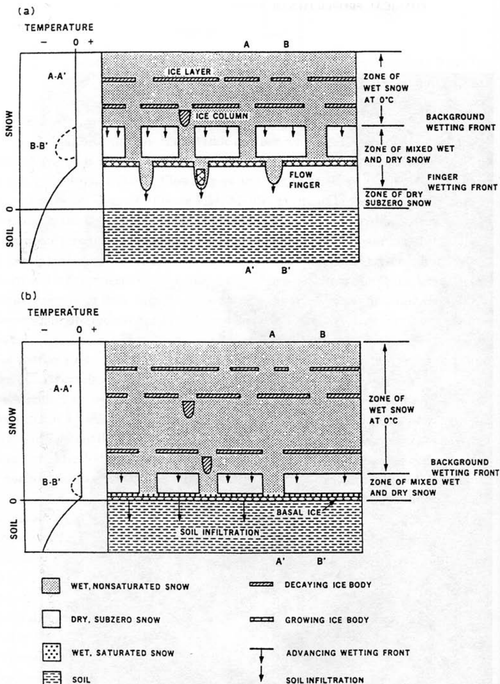
Figure 2.35. Conceptual representation of water flow, flow finger development, temperature change, and ice layer growth during meltwater percolation into an initially cold snowpack (after Marsh and Woo, 1984b). (a) Nonisothermal, before meltwater reaches the base; (b) Isothermal, after meltwater reaches the base but before the pack is fully wetted.
