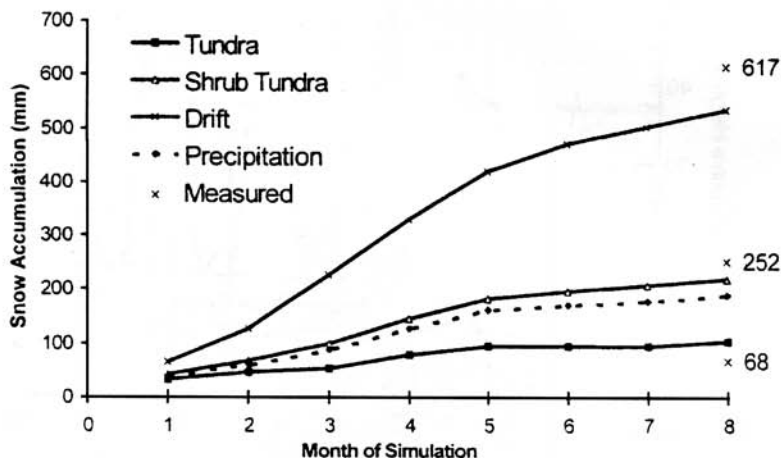
Figure 2.9. Monthly SWE accumulation for different landscape types in a lowland tundra environment, calculated by using a distributed blowing snow model. Modeled period is from October 1992 through May, 1993. Measured SWE is based on long snow surveys of depth and density conducted in early spring (Pomeroy et al., 1997a).
