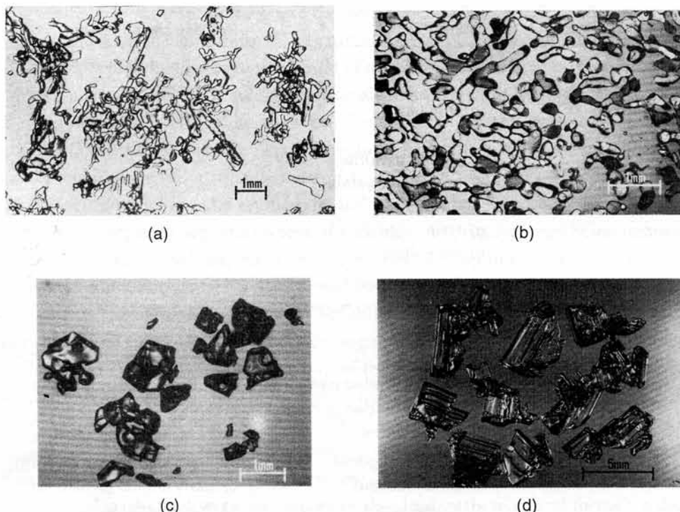
Figure 2.30. Examples of snow crystals as classified in Table 2.2 (from Colbeck et al., 1990): (a) partially decomposed fresh snow, 2a (by E. Akitaya); (b) large rounded dry grains, 3b (by E. Akitaya); (c) solid hexagonal faceted crystals, 4a (by E. Akitaya); (d) cup-shaped depth hoar crystal, 5a (by K. Izumi).
