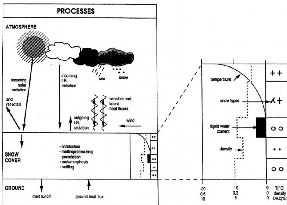
Figure 2.18. Conceptual schematic of mass and energy fluxes controlling the energetics of a snow cover and their relation to snowpack structure, properties and processes, the atmosphere, and the ground. I.R., infrared; l.w.c, liquid water content.
