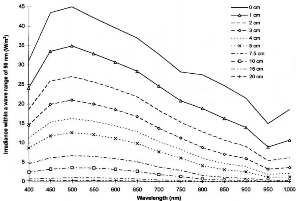
Figure 2.23. Solar irradiance within the snowpack as a function of wavelength for various depths in a clean snowpack composed of uniform spherical snow grains of 200\ \mu\text{m} diameter and a density of 200\ \text{kg m}^{-3} .
