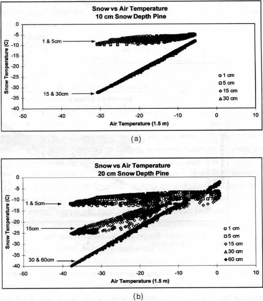
Figure 2.27. Thermal regime of a boreal forest snowpack. Temperatures measured half-hourly at various heights above the ground in Prince Albert National Park, Saskatchewan, Canada. Note that temperatures measured at heights greater than the snow depth listed for that period are air temperatures slightly above the snow surface rather than snow temperatures. (a) Early winter, 10 cm depth, 100 \text{ kg m}^{-3} density; (b) early midwinter, 20 cm depth, 150 \text{ kg m}^{-3} density; (c) midwinter, 30 cm depth, 180 \text{ kg m}^{-3} density; (d) late winter, 30 cm depth, 200 \text{ kg m}^{-3} density. Depths and densities varied over the period and values stated are approximate.
