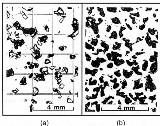
Figure 2.31. Snow structure collected at middepth from a subalpine snowpit near Banff, Alberta, by Ron Perla and photographed at a former National Hydrology Research Institute snow laboratory. Sample density is 375 \text{ kg m}^{-3} . (a) Photograph of disaggregated grains from the snow sample, displaying both faceted and rounded structure; (b) photograph of a thin-section plane prepared from the sample and showing the cross-sectional snow structure. Dark areas represent snow/ice and white areas represent pores in the snowpack (Perla, 1978)
