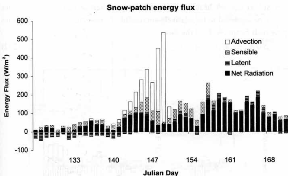
Figure 2.28. Energy fluxes for an isolated melting snowpatch in the Arctic (after Marsh and Pomeroy, 1996).
