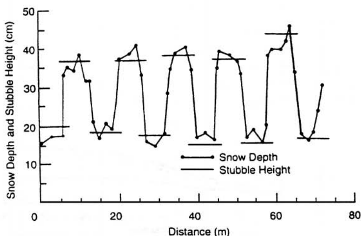
Figure 2.10. Snow depth patterns and stubble height on a wheat field harvested with alternate-height stubble management practice, southern Saskatchewan, Canada (after Pomeroy and Gray, 1995).
