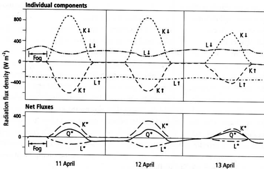
Figure 2.21. The component fluxes of incoming ( K \downarrow , L \downarrow ) and outgoing ( K \uparrow , L \uparrow ) shortwave and long-wave radiation, respectively, and the radiation balance (net) of all-wave ( Q^* ), shortwave ( K^* ), and long-wave ( L^* ) radiation during 3 days over a melting prairie snow cover. Day 1, fog then clear; day 2, clear; day 3, cloud cover (from Granger and Male, 1978).
