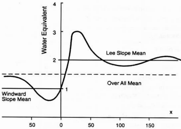
Figure 2.8. SWE deposition patterns on alpine ridges as related to windward and lee slope accumulation, near Davos, Switzerland (after Föhn and Meister, 1983).
