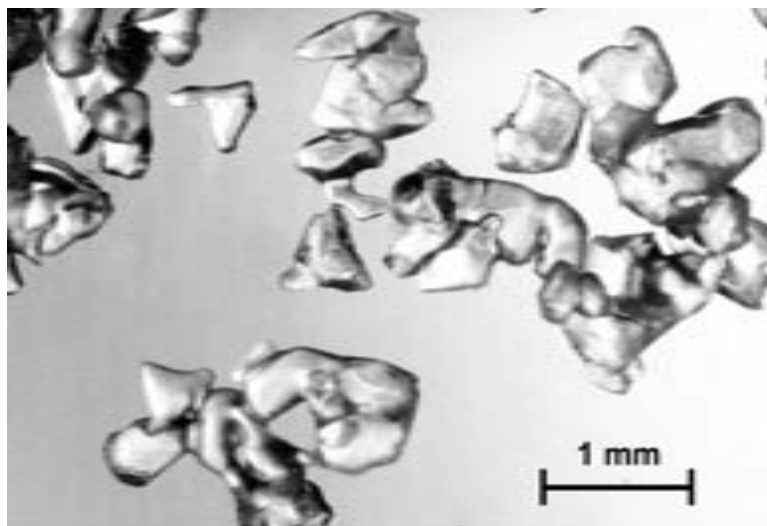
Rounding faceted particles FCxr, \varnothing (AINEVA UniMilano) #32
