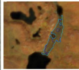
Fig. 5. Automatic segmentation of tall shrub tundra near Toolik lake
