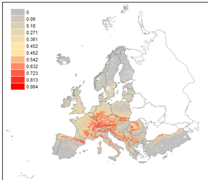
Figure 4. Suitability map of EUNIS habitat T17 (Fagus woodland on non-acid soils). The higher the suitability score the more likely the type can occur.
