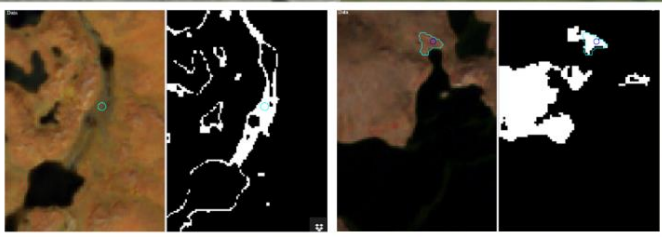
Fig. 6. Initial segmentation circle of tall shrub tundra and its homogenous area (left), and initial segmentation circle of moist graminoid tundra and its homogenous area (right) near Toolik lake
