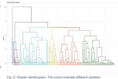
Fig. 2. Cluster dendrogram. The colors indicate different clusters.
