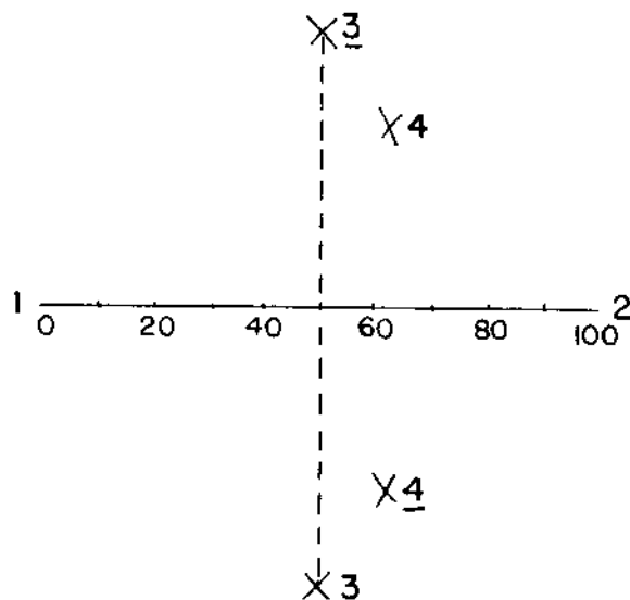
FIG. 1. Demonstration of stand location by the intersection and projection technique. Stand 3 is located at the intersection of arcs with radii of 70 units, and bases at stands 1 and 2. Its projected position on the x axis is midway between stands 1 and 2.
