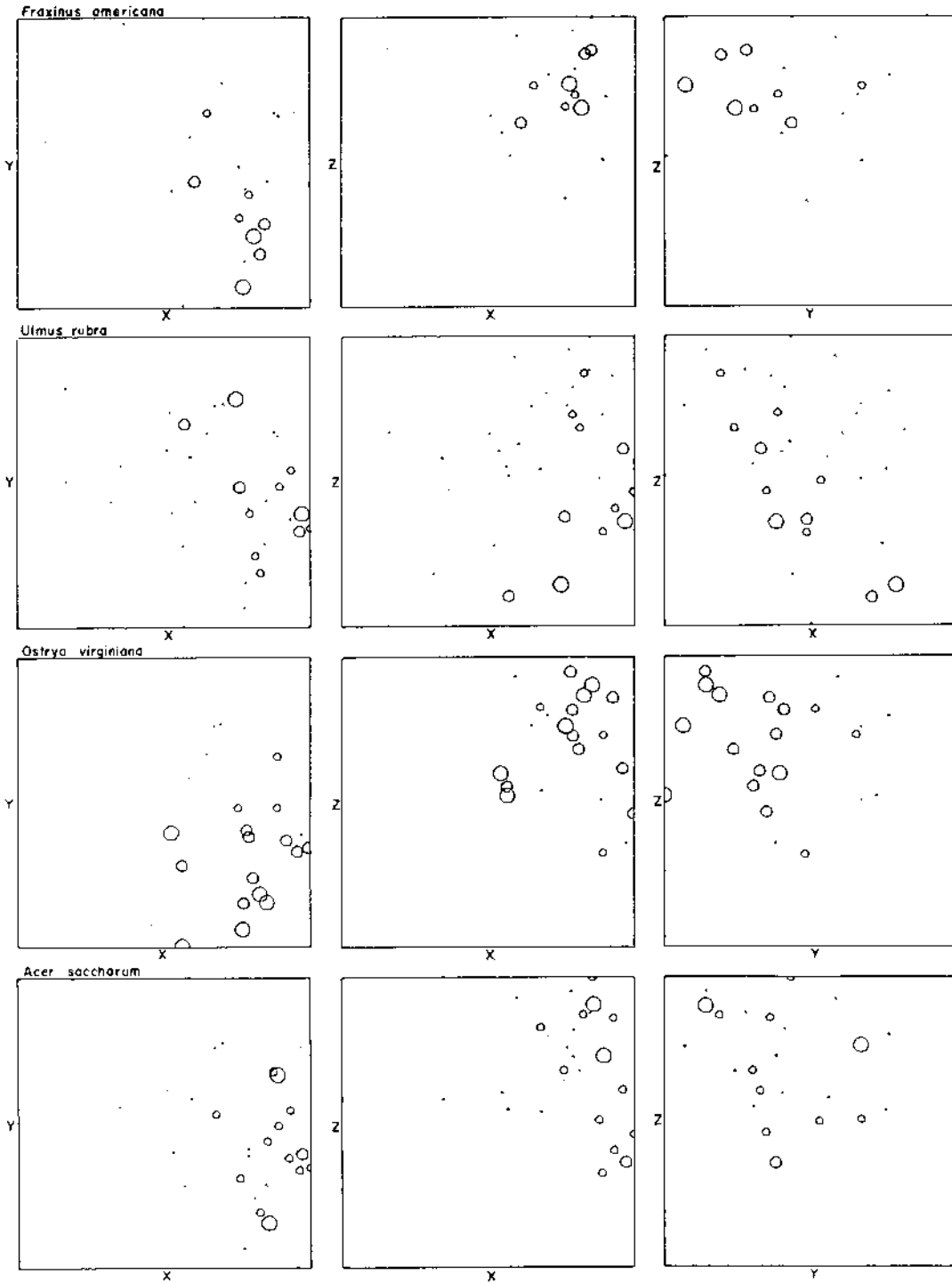
FIG. 4. Dominance behavior of the 8 most important tree species (other than Tilia americana ) within each of the 3 views of the ordination. Size of circle corresponds to the quartile size class distribution illustrated in Fig. 3. Dominance per acre at the 50% level in sq. in. is as follows: Acer saccharum 8,000; Carya orata 1,000; Fraxinus americana 2,200; Ostrya virginiana 400; Quercus alba 5,700; Quercus borealis 7,600; Quercus relativa 4,000; Ulmus rubra 3,200.
