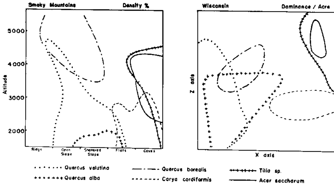
Fig. 9. View of contour drawing of trees within the x-z ordination compared with nomograms of the same or similar species in the Smoky Mountains (Whittaker 1956). Contour lines in the Wisconsin ordinations are made at the 25% (upper) size class level. Dominance values at this level in sq. in. are as follows: Acer saccharum 12,000; Carya cordiformis 400; Quercus alba 8,500; Quercus borealis 11,400; Quercus velutina 6,000; Tilia americana 5,700.
