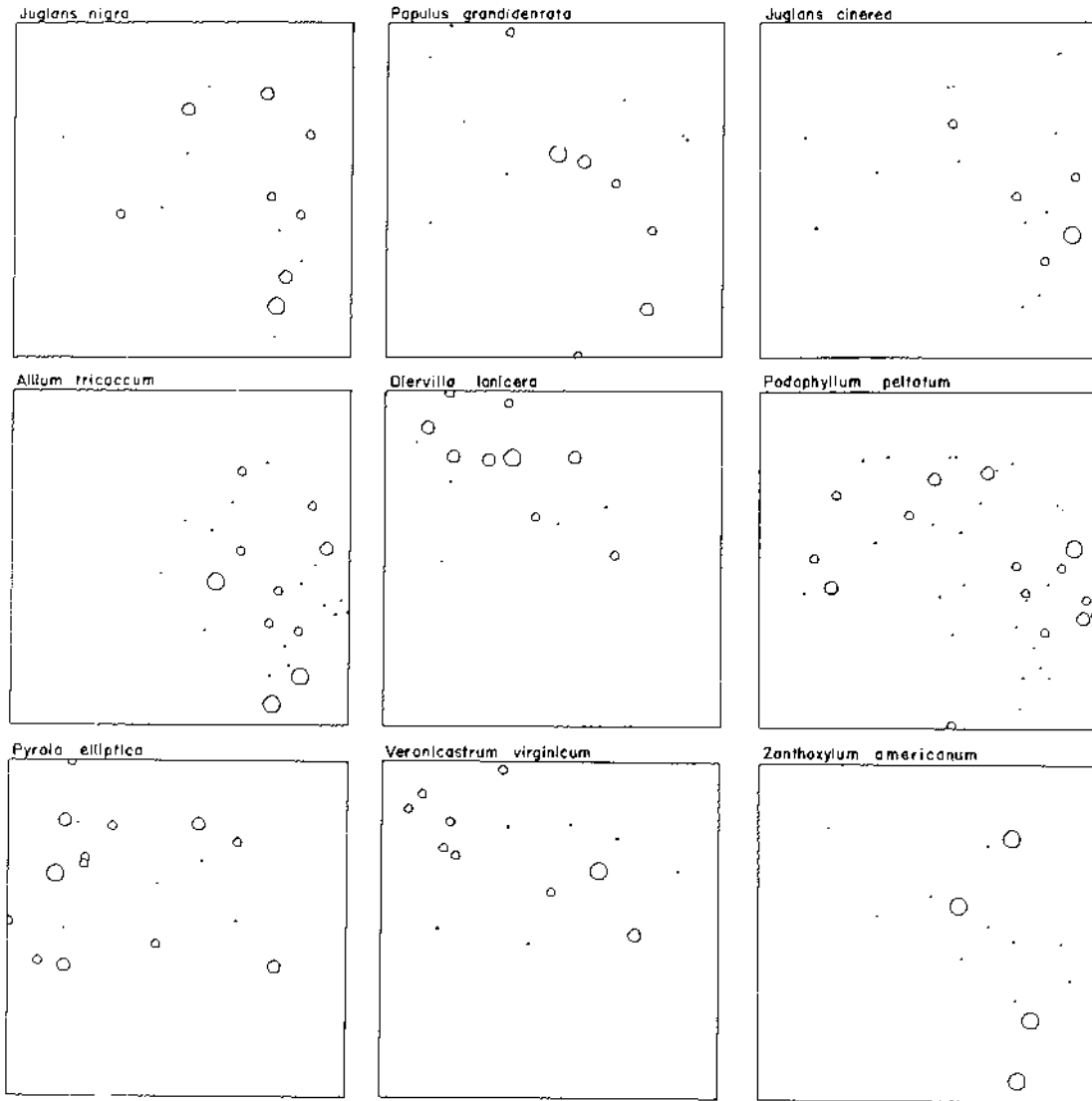
FIG. 6. Frequency behavior (understory species) and dominance behavior (trees) of 9 species not used in ordination construction. Size of circles corresponds to the quartile size class distribution illustrated in Fig. 3. Dominance per acre at the 50% level in sq. in. is as follows: Juglans cinerea 2,100; Juglans nigra 800; Populus grandidentata 1,200. Frequency at the 50% level is as follows: Allium tricoccum 10; Diervilla lonicera 10; Podophyllum peltatum 30; Pyrola elliptica 15; Veronicastrum virginicum 10; Zanthoxylum americanum 20.
