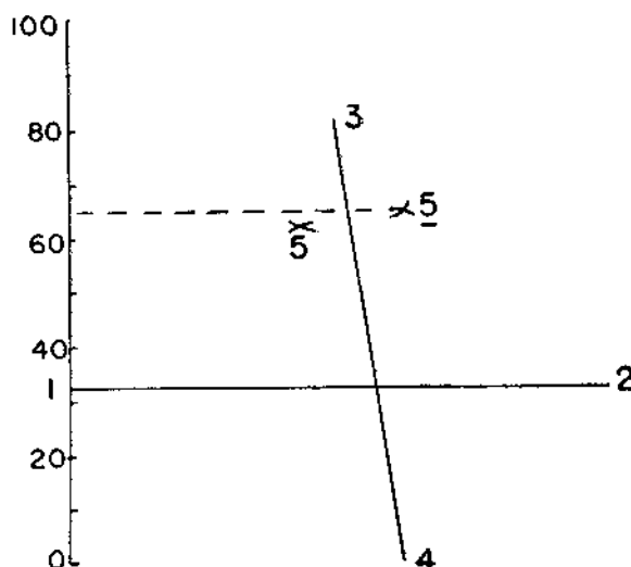
FIG. 2. Demonstration of y axis construction and stand location. Stand 5 is located at one of the two intersections of arcs 20.4 units from reference stand 3 and 64.8 units from reference stand 4. The distance of 50 units from stand 2 to stand 5 indicates the point of intersection to the right is the correct point for projection onto the y axis.
