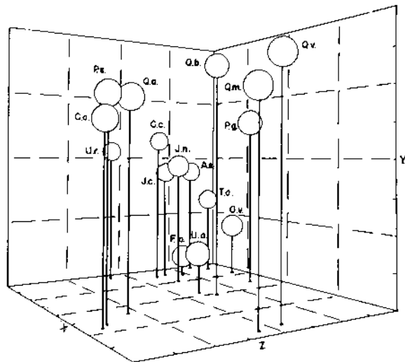
FIG. 8. Three-dimensional drawing of the center point locations of dominance behavior of tree species. Determination of center point locations explained in text. Point on frame closest to reader is lowest value for all 3 axes. The traditional position of the axes was changed to prevent the hiding of some species in the drawing.
