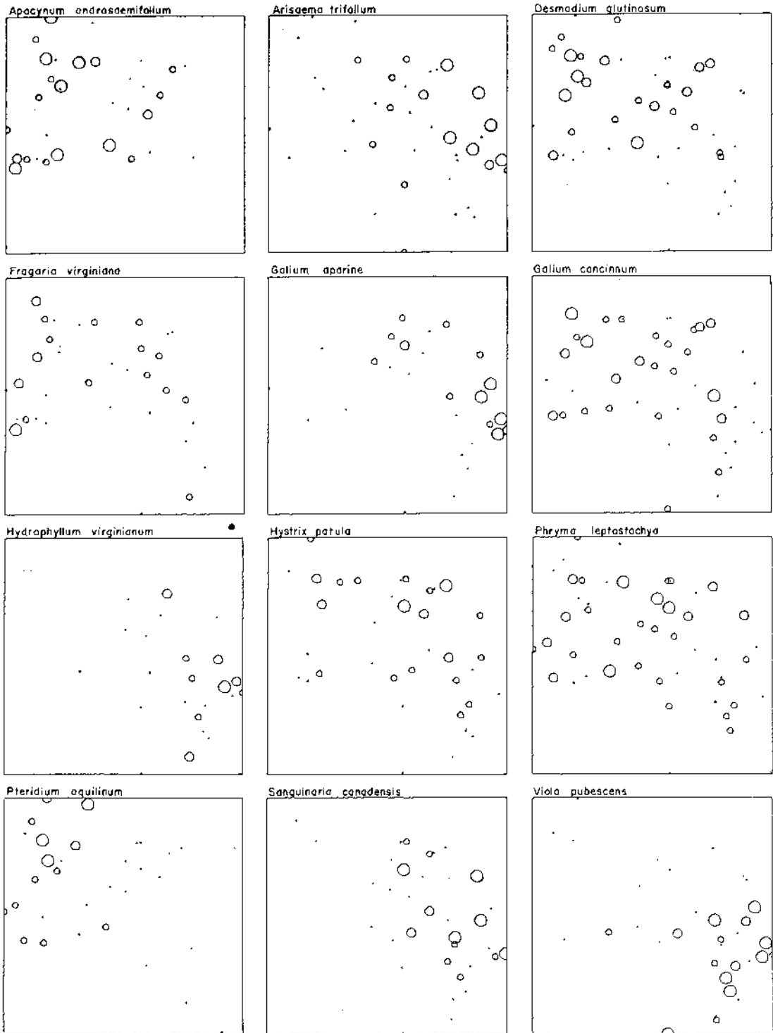
FIG. 5. Frequency behavior of score herbs (12 species) within the x-y ordination. Size of circle corresponds to the quartile size class distribution illustrated in Fig. 3. Frequency at the 50% level is as follows: Apocynum androsaemifolium 10; Arisaema trifolium 30; Desmodium glutinosum 40; Fragaria virginiana 25; Galium aparine 50; Galium concinnum 47; Hydrophyllum virginianum 25; Hystrix patula 10; Phryma leptostachya 30; Pteridium aquilinum 27; Sanguinaria canadensis 35; Viola pubescens 37.
